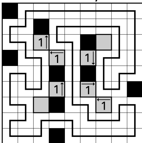
9. No Touch Yajilin
